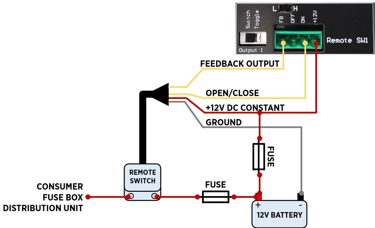
Figure 9: Switch signal type of remote switch.
