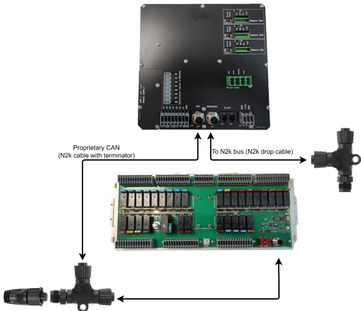
Figure 11: Connecting the panel to the distribution unit and NMEA2000 network.
