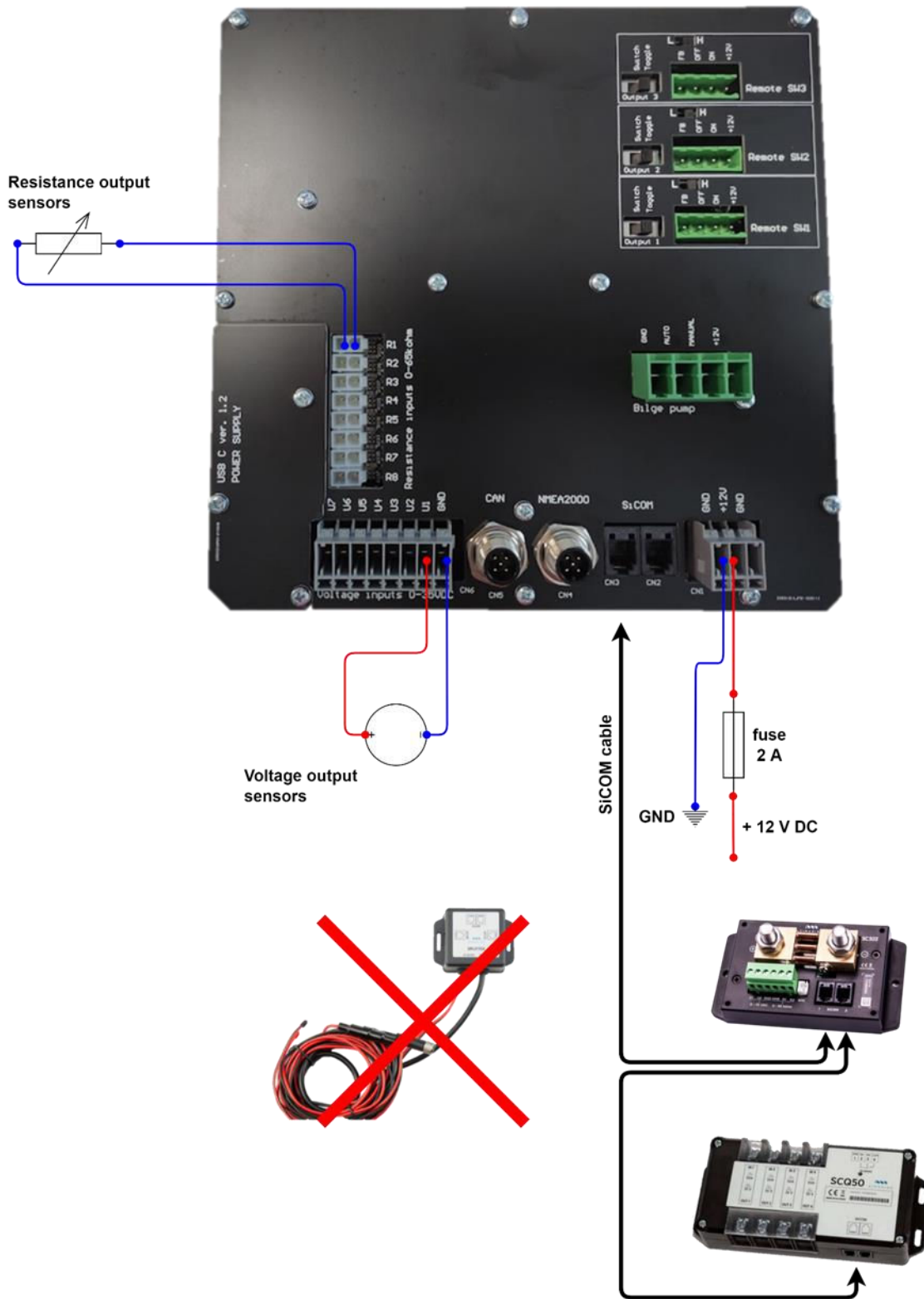
Figure 3: Control panel connections diagram.
