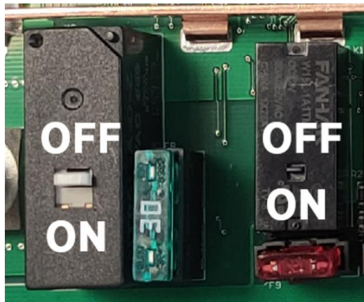
Figure 15: Tabs on relays for manual switching.
