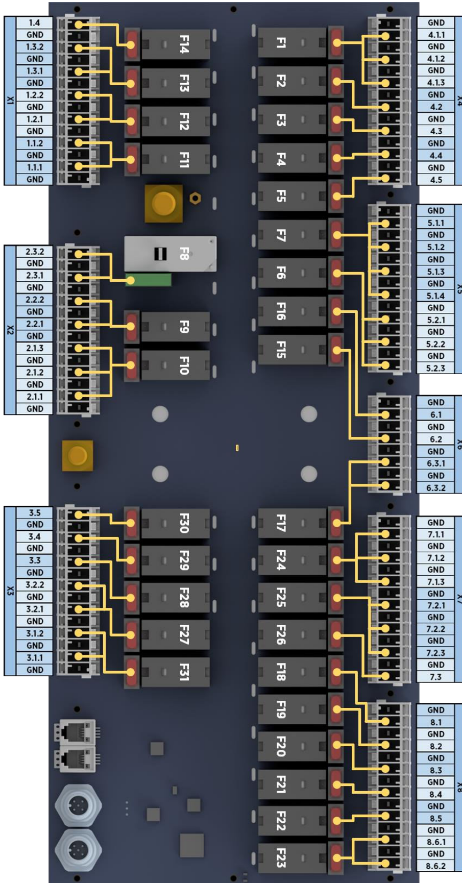
Figure 14: Relays with corresponding pins.
