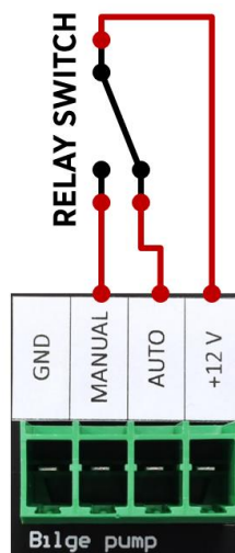
Figure 5: Internal schematics of the bilge pump connector.
