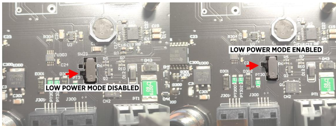
Figure 2: Low power mode enable/disable switch.
