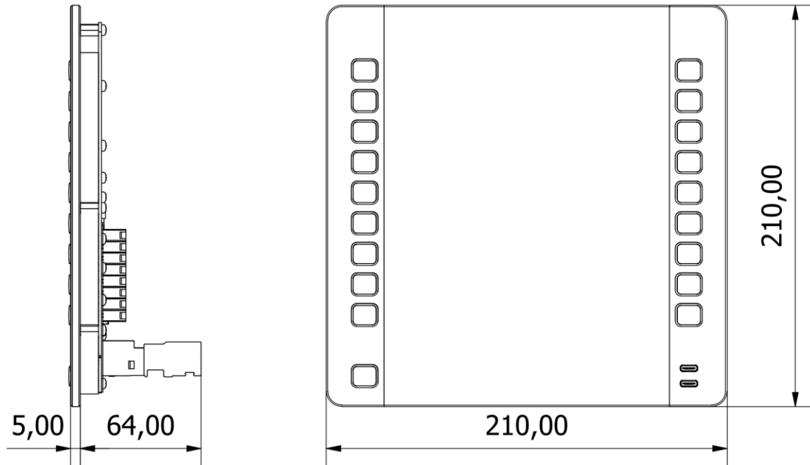
Figure 19: Nereide 2 general dimensions.
