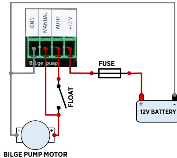
Figure 4: Connecting a bilge pump.
