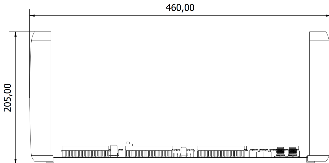
Figure 21: SPU303 dimension with open covers.
