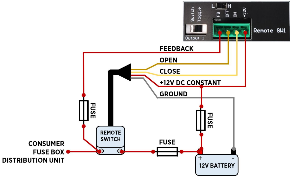
Figure 10: Feedback signal from remote switch output.
