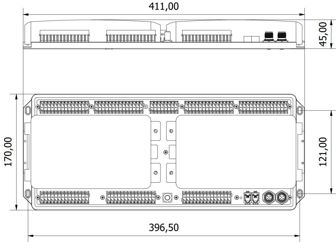
Figure 20: SPU303 DC Distribution Unit general dimensions.
