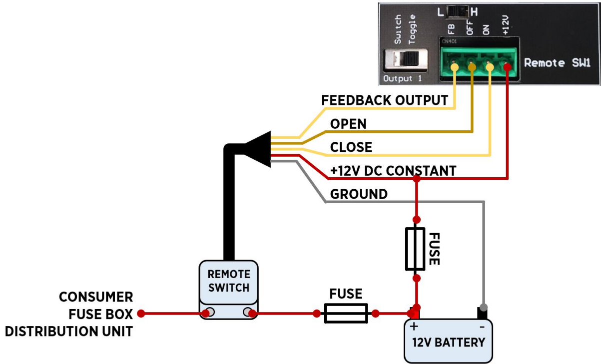
Figure 8: Toggle signal type of remote switch.
