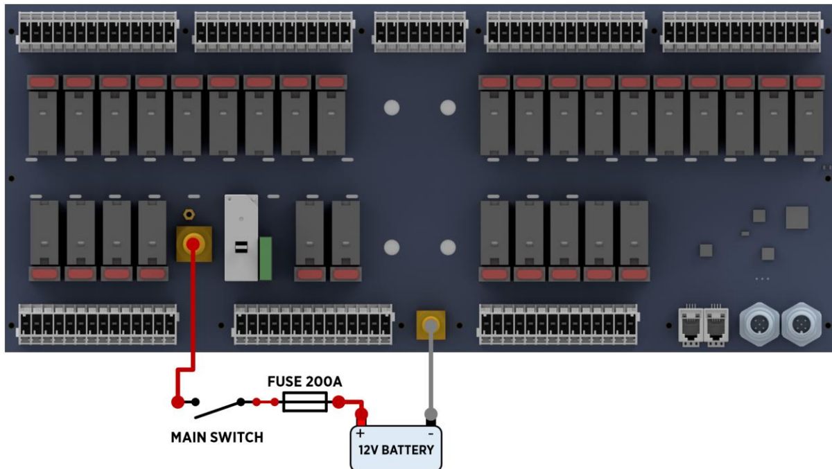
Figure 13: Power source for the DC distribution unit.
